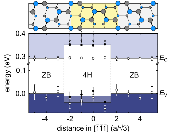
Figure 4. Conduction and valence band edge positions determined for the measured Sb compositions shown in figure 3 using the Sb composition bowing parameters of \text{InAs}_{1-x}\text{Sb}_x given in [31] (white symbols). In addition, near the twin boundary, the stacking corresponds to a 4H wurtzite structure insertion, which additionally has band offsets with the surrounding zincblende structure [34]. This shifts the band edge positions upward, changing the almost flat band condition from the conduction to the valence band (see filled symbols). The averaged band alignment is indicated by the background shading.
