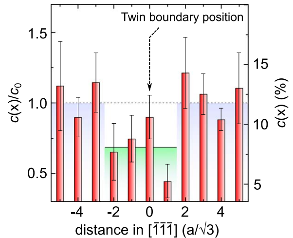
Figure 3. Normalized, plane-resolved concentration c(x) of Sb atoms in \text{InAs}_{0.90}\text{Sb}_{0.10} NWs as a function of the distance x to a twin boundary. The concentrations were measured in STM images of the \{110\} sidewall facet. Values above (below) 1 indicate a higher (lower) than statistically expected occurrence of Sb. Four atomic planes round the twin boundary exhibit a significantly smaller Sb concentration than statistically expected (see green shaded area). The average normalized Sb concentration near the twin boundary is 0.68 \pm 0.1 , corresponding to \text{InAs}_{0.92}\text{Sb}_{0.08} .
