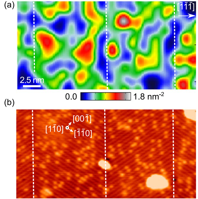
Figure 2. (a) Local Sb surface concentration map derived from the STM image shown in (b). (b) Atomically resolved constant-current STM image of the sidewall surface measured at 77 K ( -3 \text{ V} sample voltage and 10 \text{ pA} tunnel current). The image shows the filled dangling bond states above the surface anions. The atomically-sized protrusions arise from Sb atoms incorporated on anion sites. Twin boundaries are marked by dashed vertical lines.
