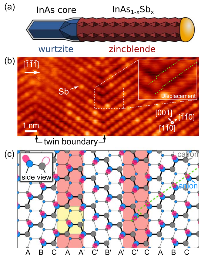
Figure 1. (a) Schematic of the zincblende \text{InAs}_{1-x}\text{Sb}_x nanowire (red), grown on top of wurtzite \text{InAs} nanowire (blue) in [\bar{1}\bar{1}\bar{1}] direction. During the growth of the top part, a lateral overgrowth of the \text{InAs} bottom part can be observed. (b) Atomically resolved constant-current STM image of two twin boundaries at the \text{InAs}_{0.90}\text{Sb}_{0.10} NW sidewall measured at 77 K ( -2 V sample voltage and 700 pA tunnel current). The image shows the filled dangling bond states above the surface anions. The bright atomically localized contrast features arise from Sb atoms incorporated on anion sites. Inset: magnification of one of the twin boundaries. One chain of dangling bonds in [\bar{1}\bar{1}0] direction is marked by green dashed lines. If one traces this chain back to the twin boundary, the dangling bond imaged directly at the boundary exhibits a slight downward displacement. The displacement implies a directional change of the dangling bond at the twin boundary. (c) Ball-model of the ZB atomic lattice of the \{110\} NW sidewall facet including two twin boundaries (red shaded areas). In (As) atoms of the first and second atomic layer are represented by filled gray (blue) circles. The dangling bonds of the As atoms in the first atomic layer are shown as red ellipsoids. For the formation of a twin boundary, the insertion of a single WZ layer is necessary. The a -plane unit cell of the WZ layer is shown by the yellow shaded rectangle. Inset: side view along [110] direction, showing the orientation of both, filled (red filled ellipse) and empty (empty ellipse) dangling bonds at the anions and cations, respectively.
